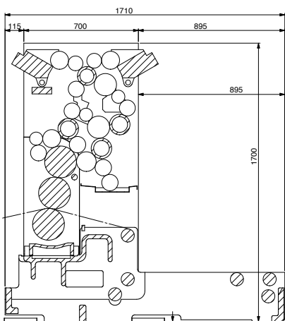
Novaprint print unit (double ink tray optional)
